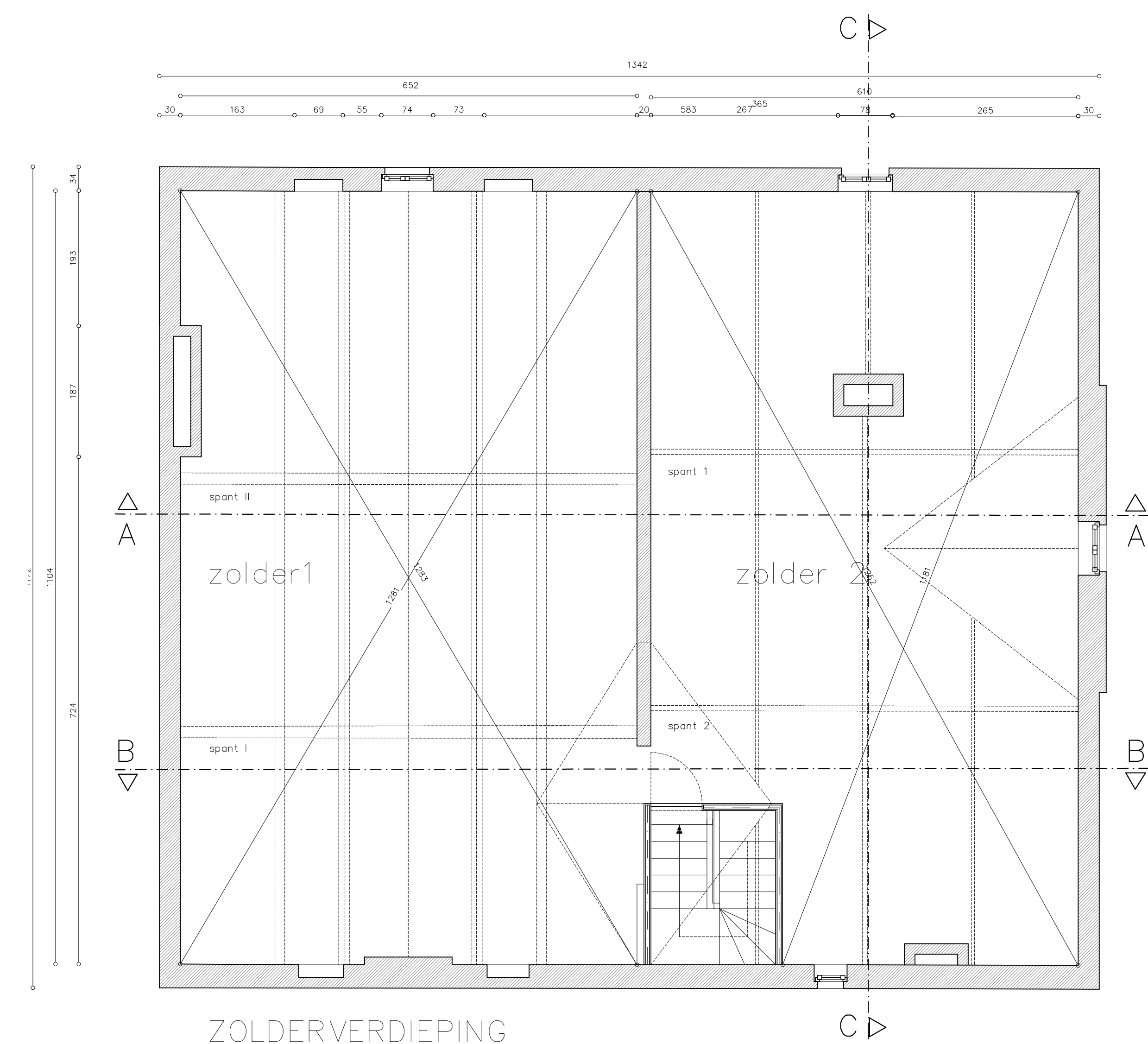
ZOLDERVERDIEPING
