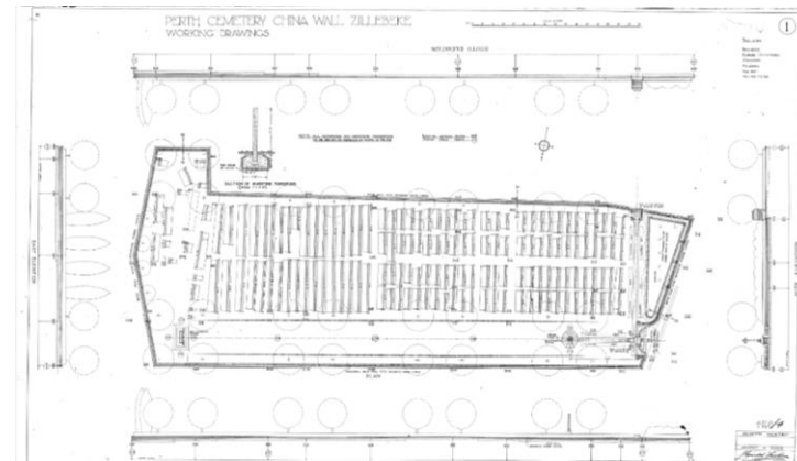
Figuur 2. Perth Cemetery China Wall, working drawings 7
