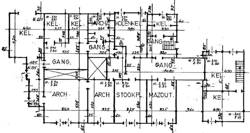
Plantekeningen Hotel Schaetzen (d.d. 12/01/1982), detail kelder
