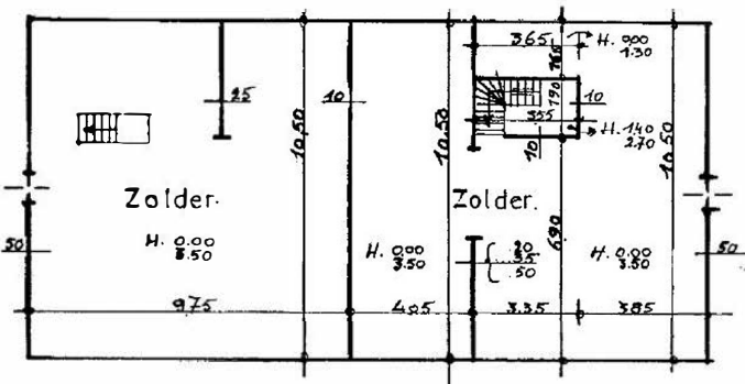
Plantekeningen Hotel Schaetzen (d.d. 12/01/1982), detail zolder
